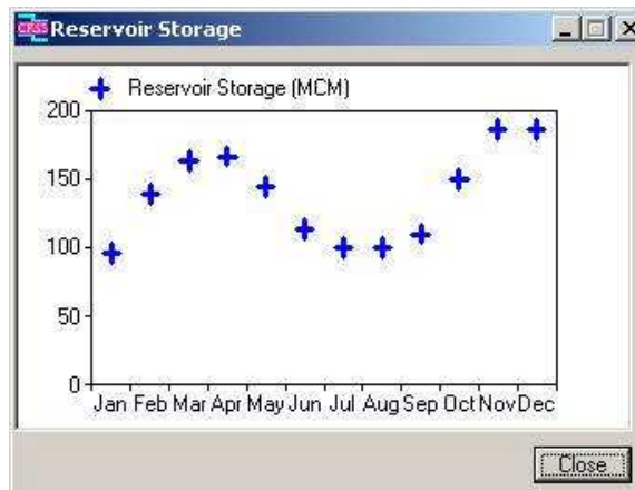
Figure 5.30 Variation of reservoir storage – Type 2
