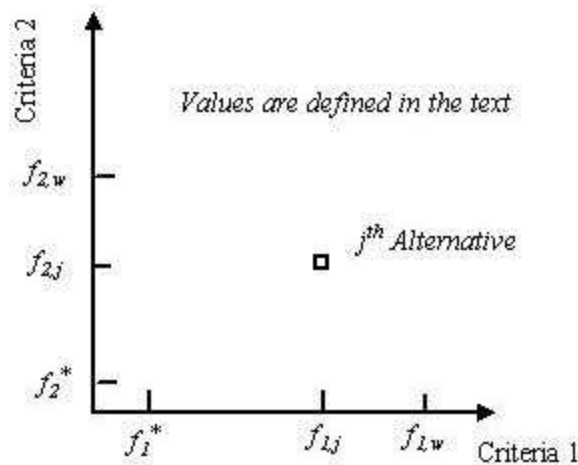
Figure 3.3 Values used to determine distance metric for an alternative
