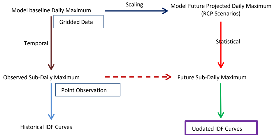
Figure 3: Concept of equidistance quantile matching method for updating IDF curves
