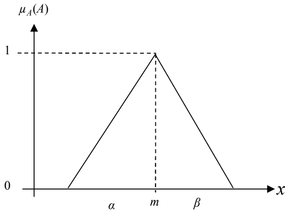
Figure 2.3. Triangular membership function of L-R fuzzy number
