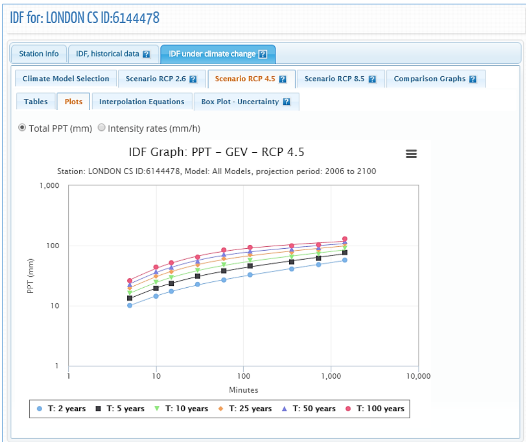
Figure 63. Total precipitation (in mm) updated IDF graph for different return periods
