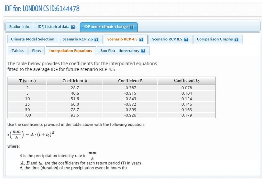
Figure 65. Fitted IDF equation for future scenario
