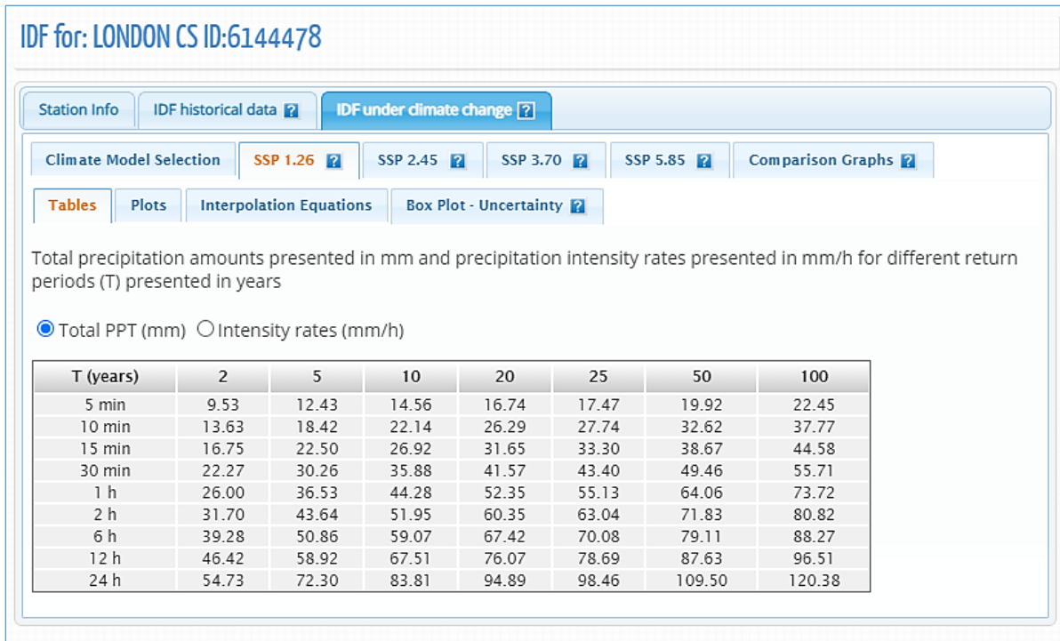
Figure 60. Updated IDF tables for future climate conditions – total precipitation in mm using CMIP6 GCMs
