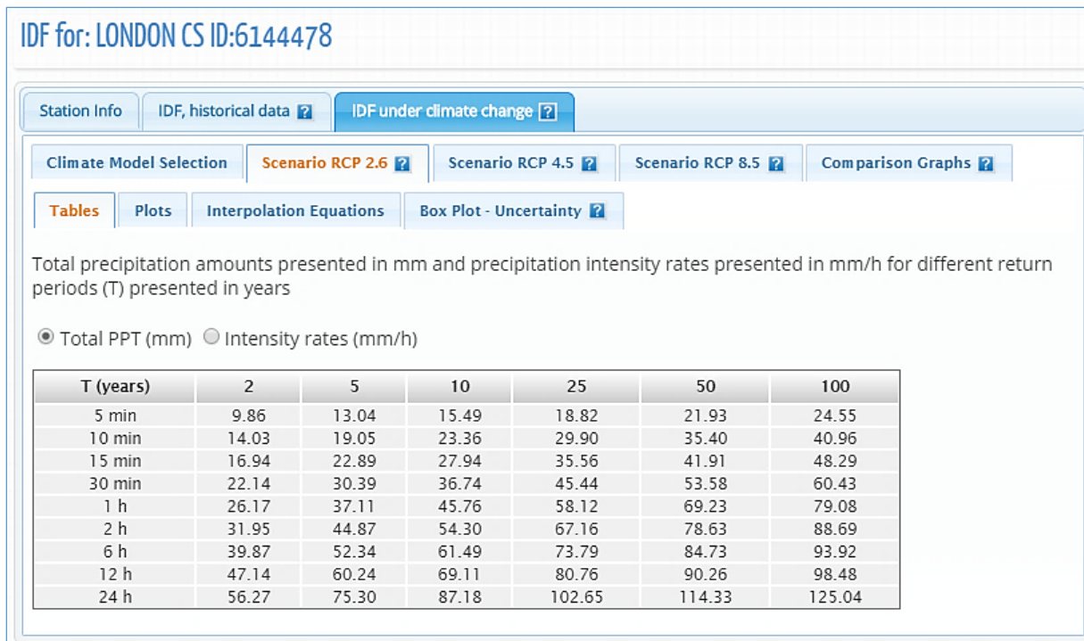
Figure 61. Updated IDF tables for future climate conditions – total precipitation in mm using CMIP5 GCMs
