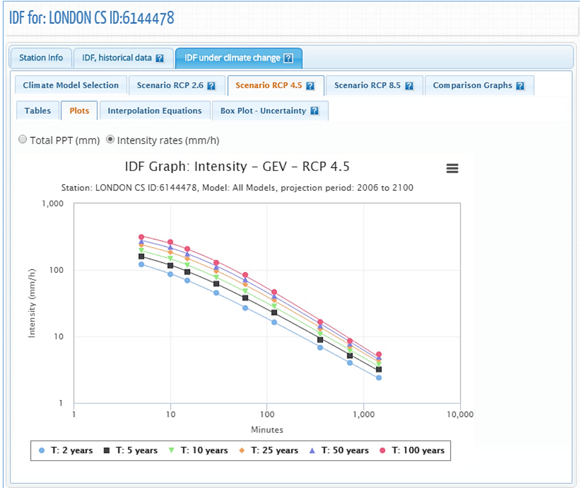
Figure 64. Rainfall intensity (in mm/h) updated IDF graph for different return periods
