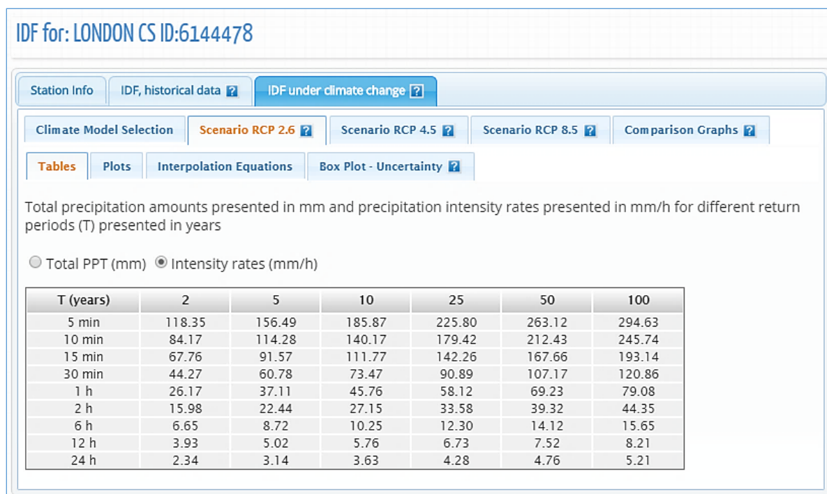
Figure 62. Updated IDF tables for future climate conditions – rainfall intensity in mm/h
