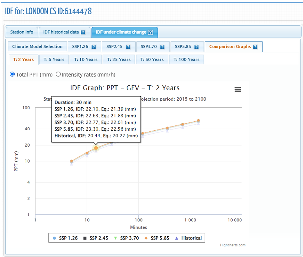
Figure 68. IDF comparison graphs
