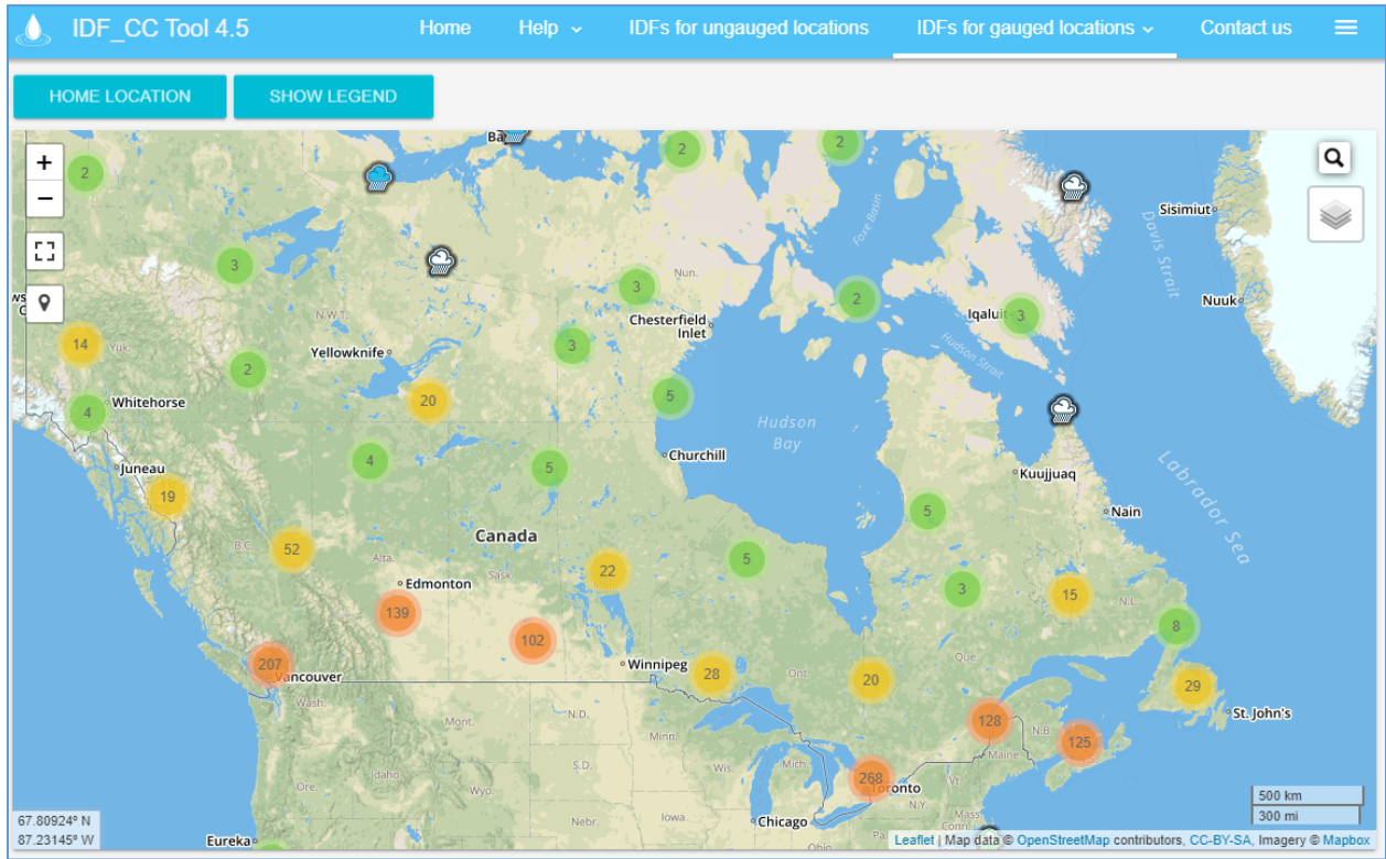
Figure 2. Screenshot of the IDF_CC tool version 5.0 user interface
