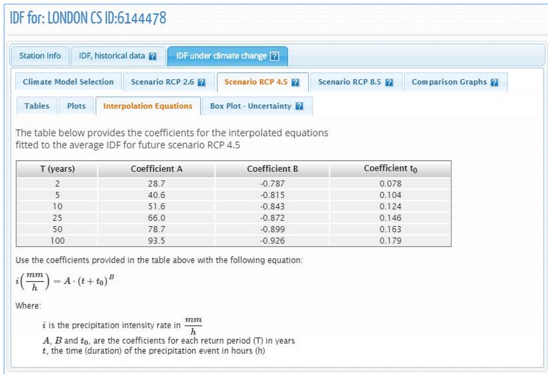
Figure 64. Fitted IDF equation for future scenario
