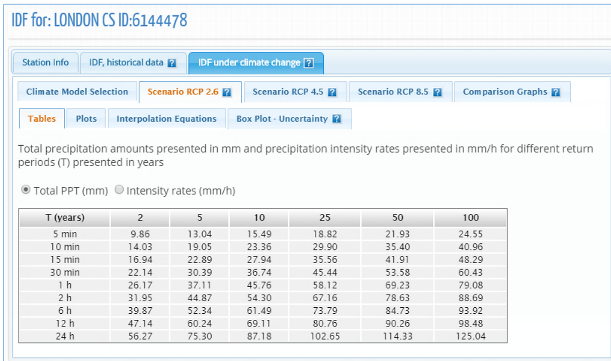
Figure 60. Updated IDF tables for future climate conditions – total precipitation in mm using CMIP5 GCMs
