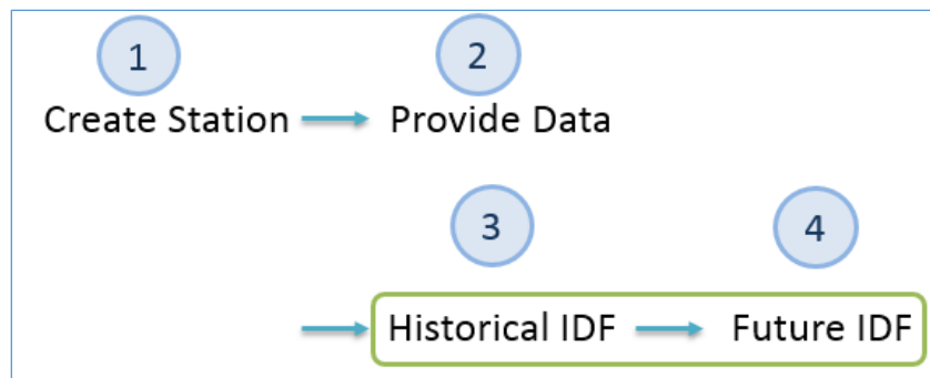
Figure 69. Updating IDF for future climatic conditions for a user provided station
