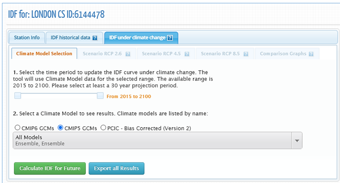
Figure 58. Selection of CMIP5 or Bias corrected CGM model and projection period
