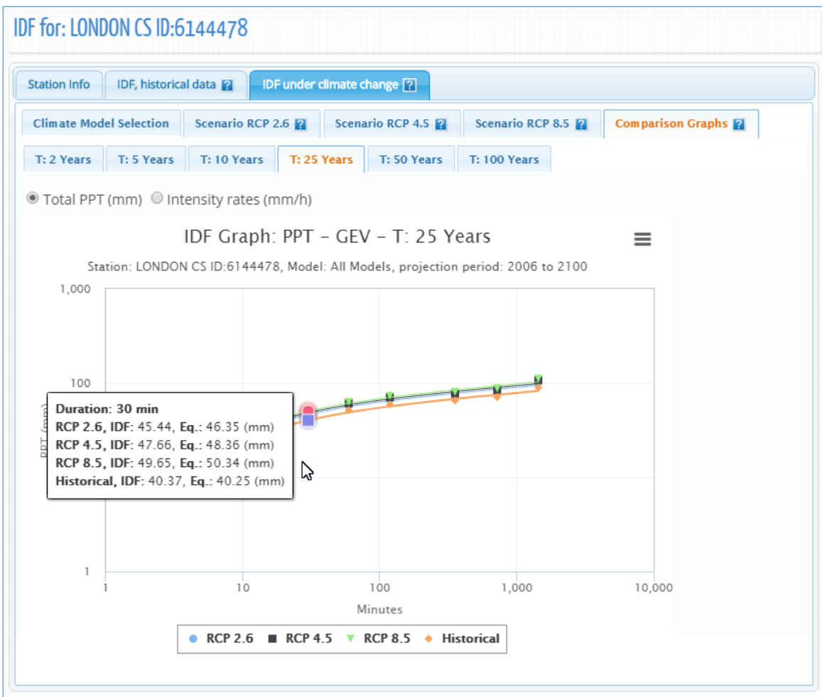
Figure 67. IDF comparison graphs
