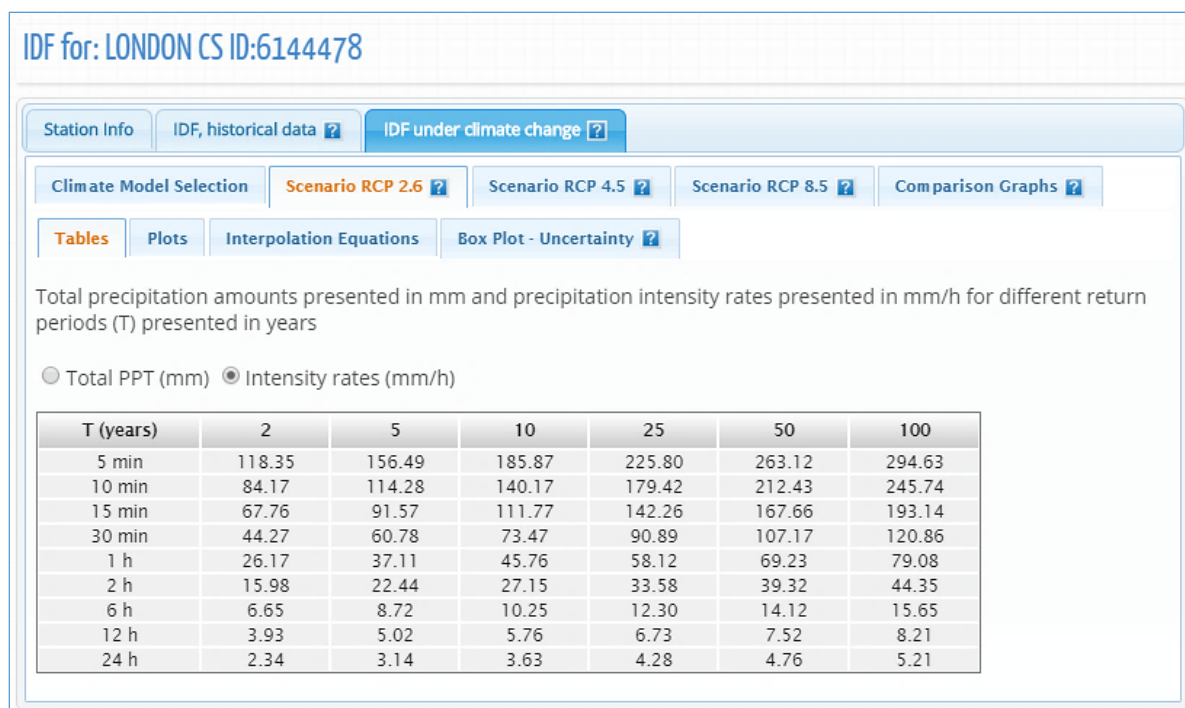
Figure 61. Updated IDF tables for future climate conditions – rainfall intensity in mm/h
