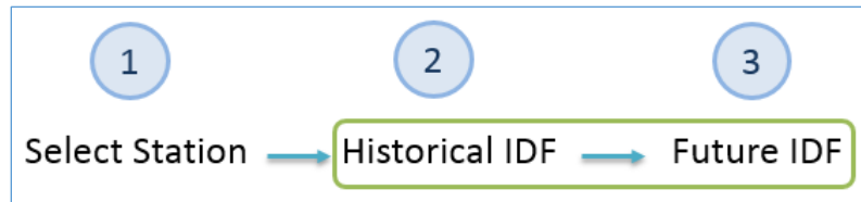
Figure 68. Updating IDF curves for future climatic conditions for an Environment Canada station
