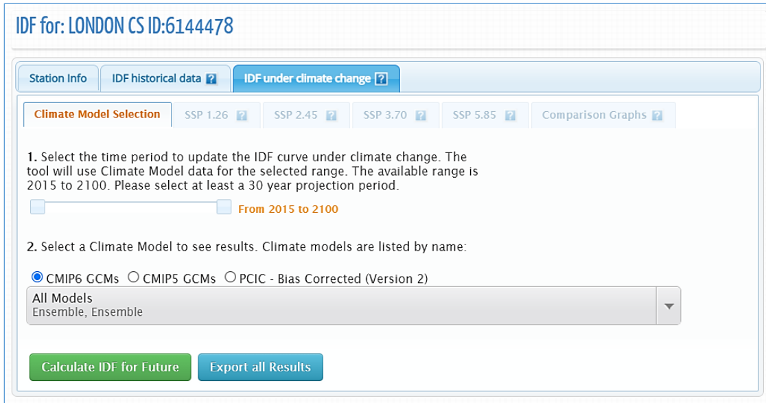
Figure 57. Selection of the CGM CMIP6 model and projection period
