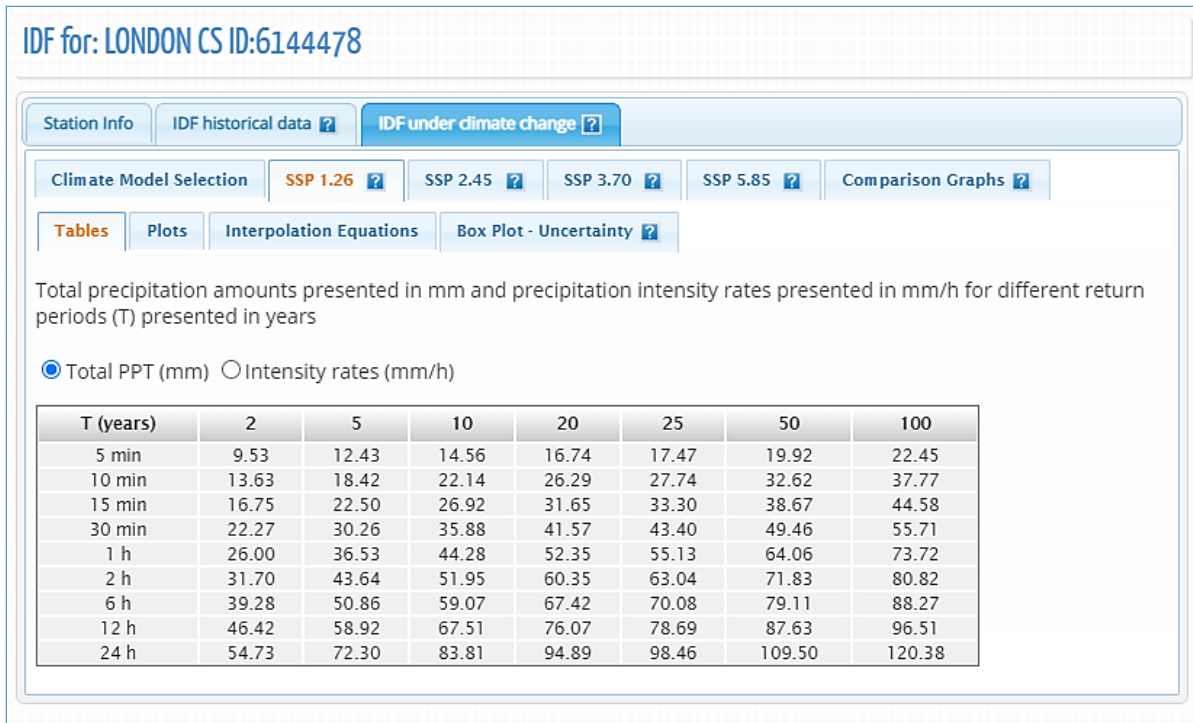
Figure 59. Updated IDF tables for future climate conditions – total precipitation in mm using CMIP6 GCMs
