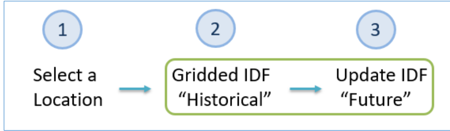
Figure 70. Updating IDFs for future climatic conditions for a selected location within Canada (Gridded IDFs)
