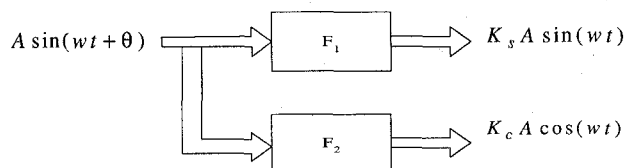
Fig 1. Output of the orthogonal digital filters.
