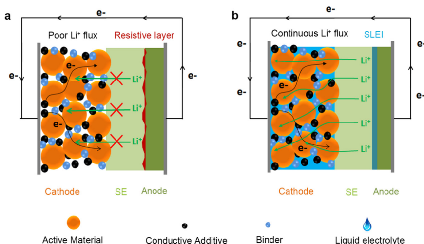
Fig. 1. Schematic diagram of 3D continuous Li + ion flux. (a) Illustration of lithium ion and electron fluxes inside the conventional cathode. (b) A trace amount of LE was added to both sides of the SE, filling the pores within the cathode as well as wetting the Li metal surface.
