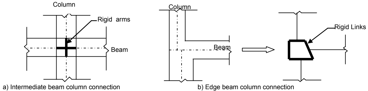
Figure 3. Rigid arms for modeling of beam-column connections
