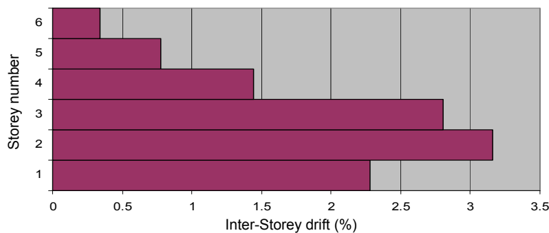
Figure 6. Interstorey drift distribution at collapse
