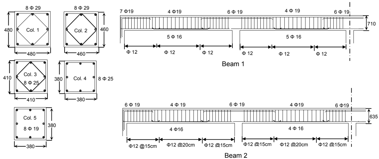
Figure 2. Reinforcing details
