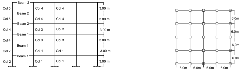
Figure 1. Six-Storey building
