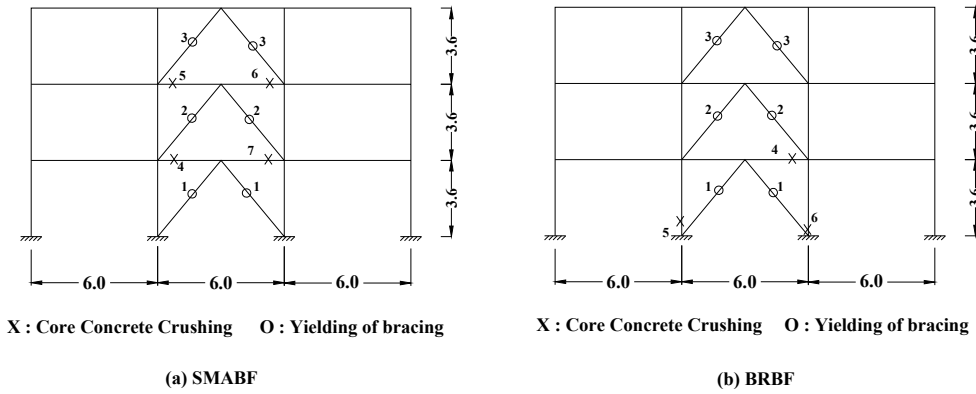
Figure 11: The sequence of brace yielding and core concrete crushing at PGA= 0.75g
