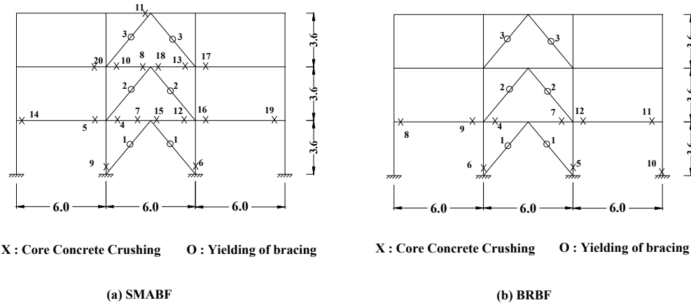
Figure 12: The sequence of brace yielding and core concrete crushing at PGA= 1.00g
