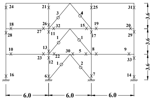
X : Core Concrete Crushing O : Yielding of bracing (a) BRBF
