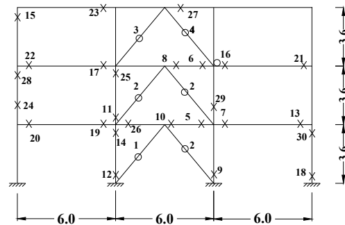
X : Core Concrete Crushing O : Yielding of bracing (b) SMABF
