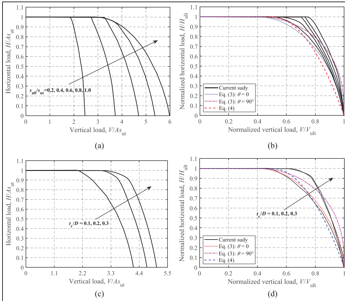
Figure 8. H - V failure envelopes: (a) dimensionless, s_{u0}/s_{ut} = 0.2 – 1.0 and t_c/D = 0.2 , (b) normalized, s_{u0}/s_{ut} = 0.2 – 1.0 and t_c/D = 0.2 , (c) dimensionless, s_{u0}/s_{ut} = 0.6 and t_c/D = 0.1 – 0.3 , and (d) normalized, s_{u0}/s_{ut} = 0.6 and t_c/D = 0.1 – 0.3 .
