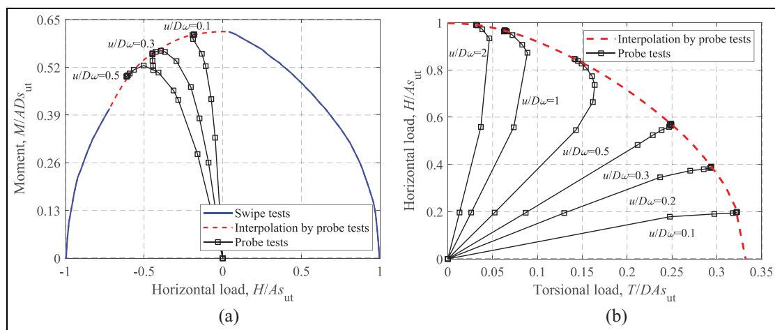
Figure 4. M-H and H-T failure envelopes for a uniform soil at V/V_{ult} = 0.50 : (a) M-H and (b) H-T.
