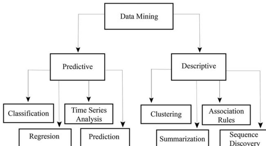
FIGURE 2 Data mining models and task 44
